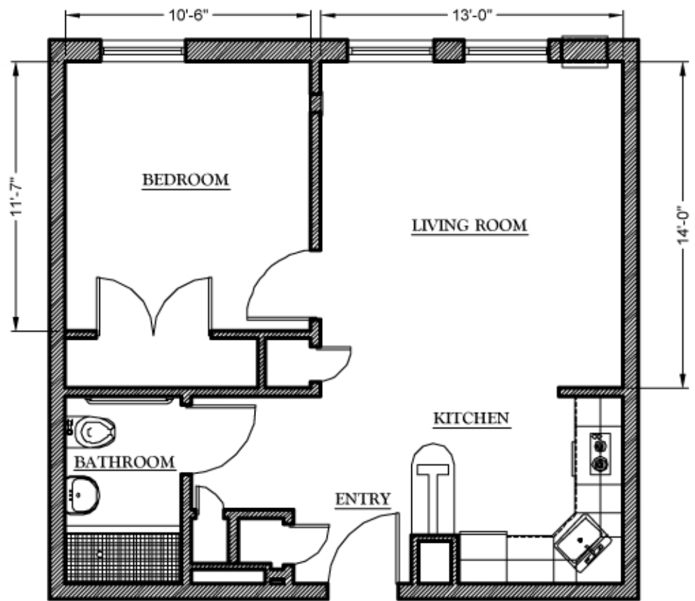
One Bedroom Floor Plan - 16 Line / Type D-1 Not To Scale
